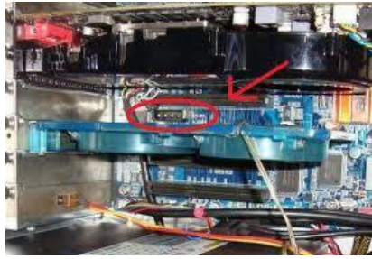
Gambar 49. Jumper VGA
