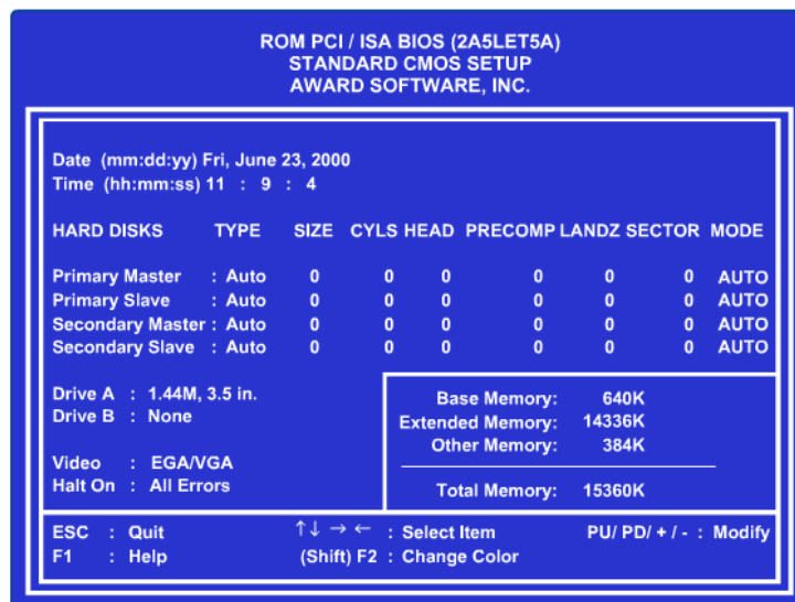
Gambar 77. Tampilan Setup CMOS standar
